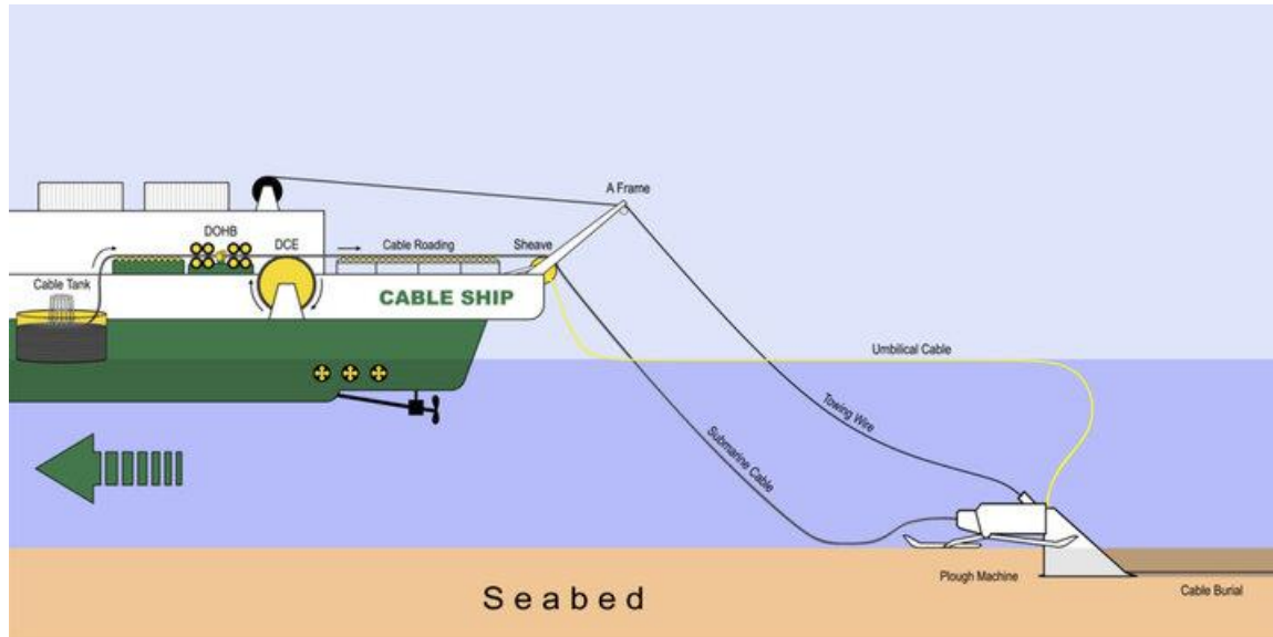
Fonte: https://stock.adobe.com/search/images?k=%22submarine+cable%22
